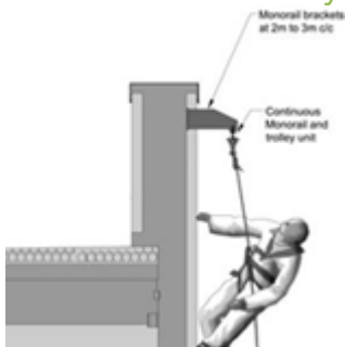
Eye bolt suspension system
